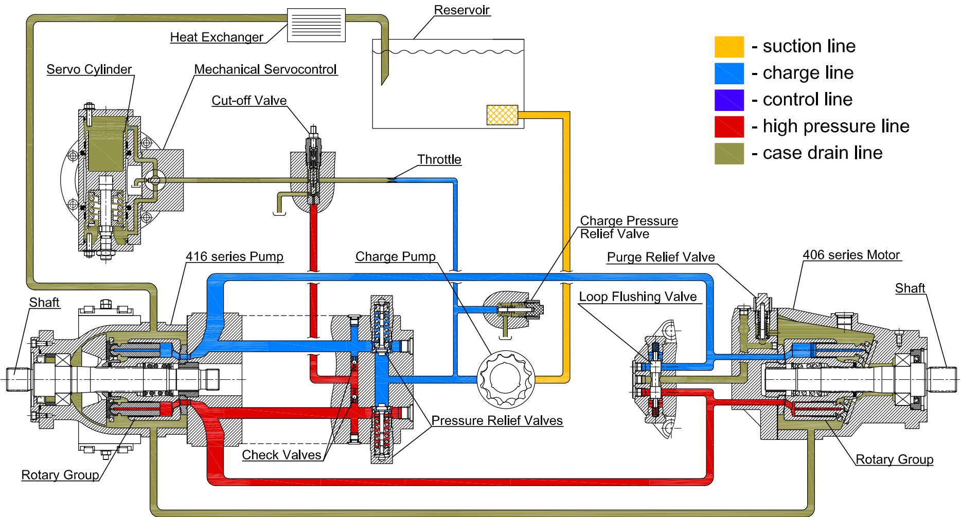
Forward Position of Swashplate in the pump. Cut-off valve operation.
